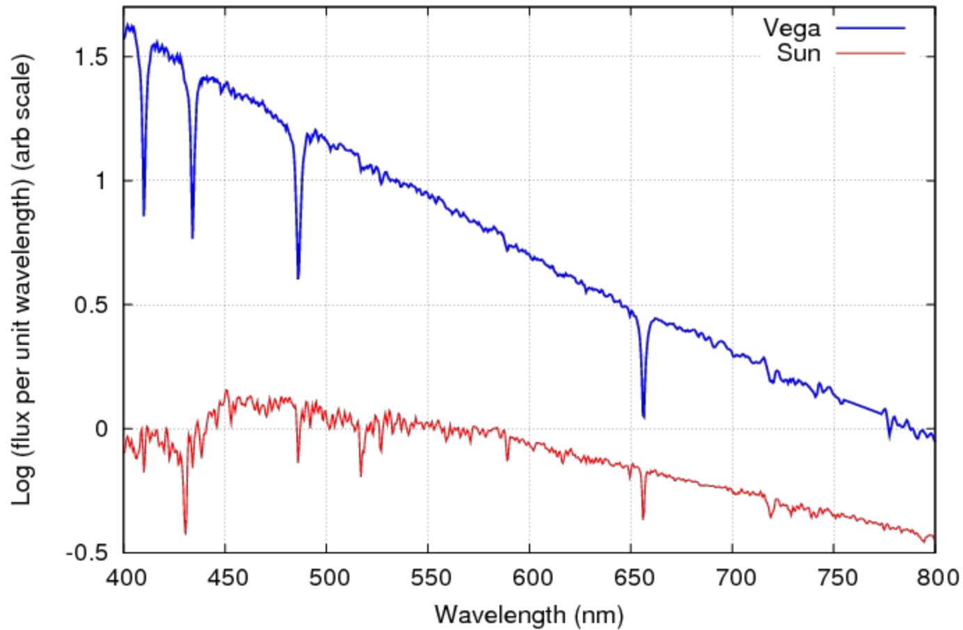
Spectra of two stars
